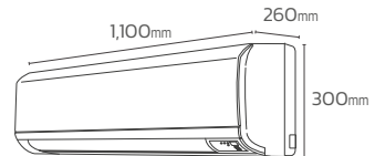
RPK-2.5-4.0FSN4M 15kg
