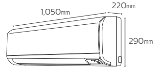
RPK-2.5-4.0FSN4M 15kg
